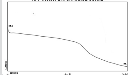
XPP-5466R PERFORMANCE CURVE
